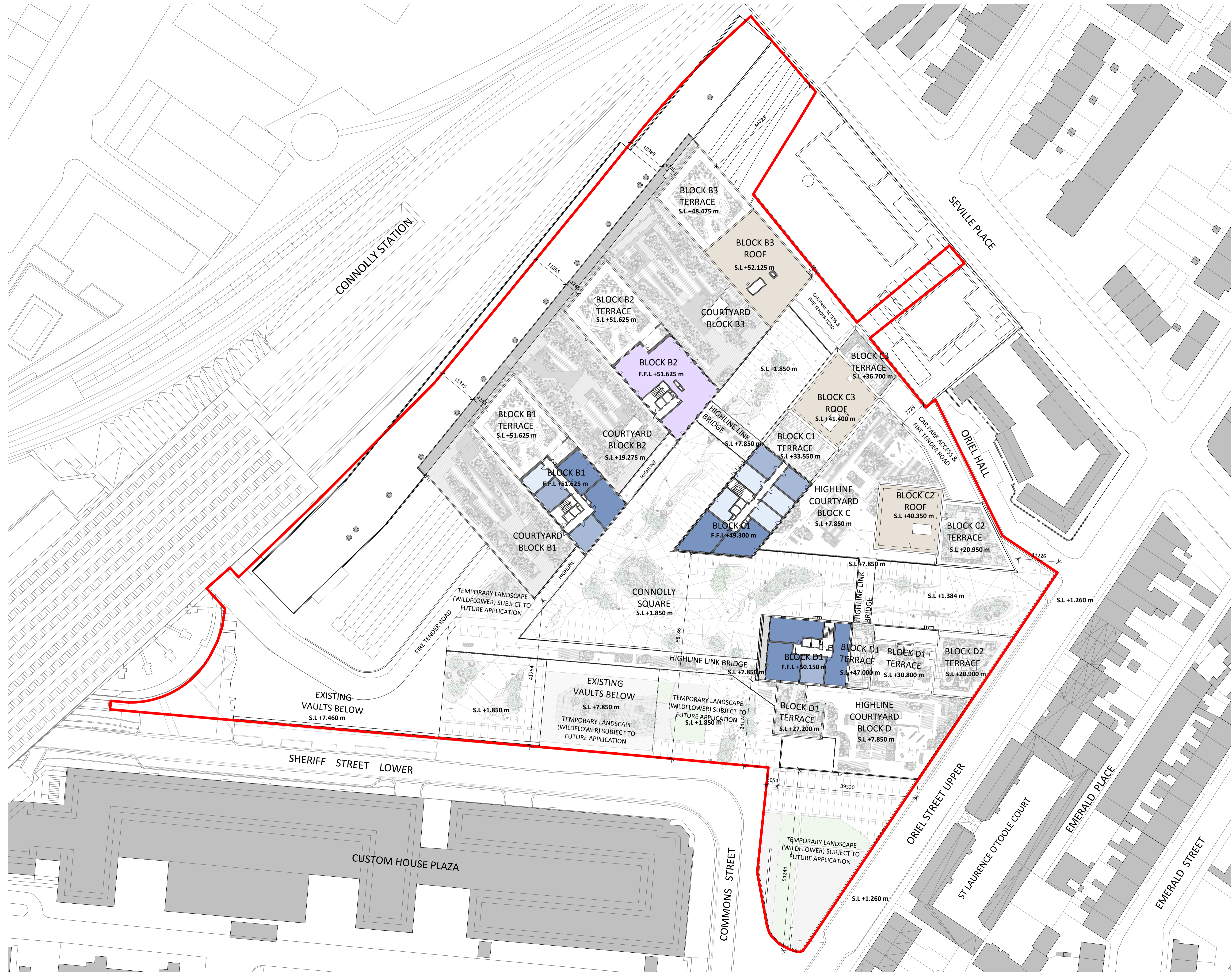
1 SITE LAYOUT PLAN - LEVEL 14 1:500
